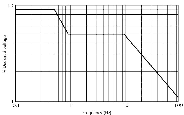
Figure 16 - Voltage levels of signals used in public MV distribution systems [11]
