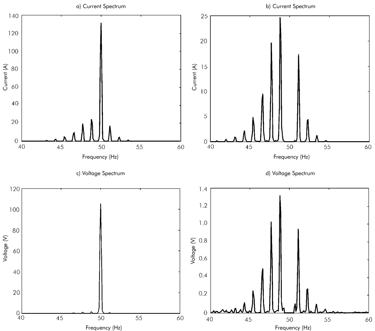
Figure 2 - Results of the spectral analysis of the motor phase current and voltage at the motor terminals
