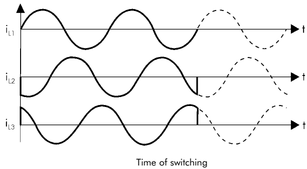
Figure 6 - Waveforms of currents in a three-phase configuration with a neutral conductor for integral cycle control
