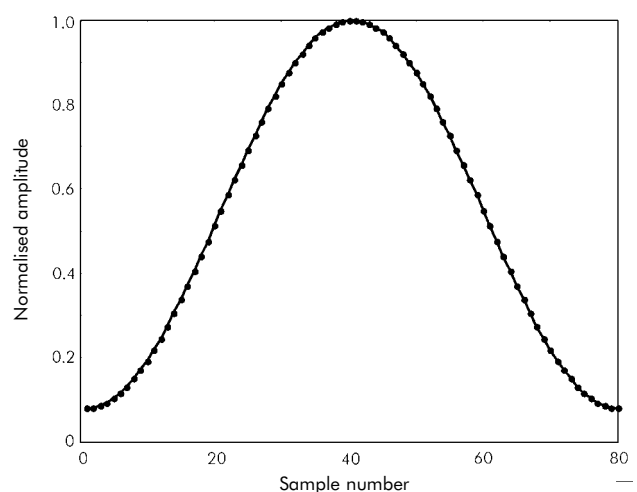
Figure A.1.6c - Hamming window
