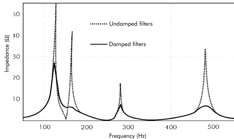
Figure 17 - Example of impedance seen from converters' terminals [10]
