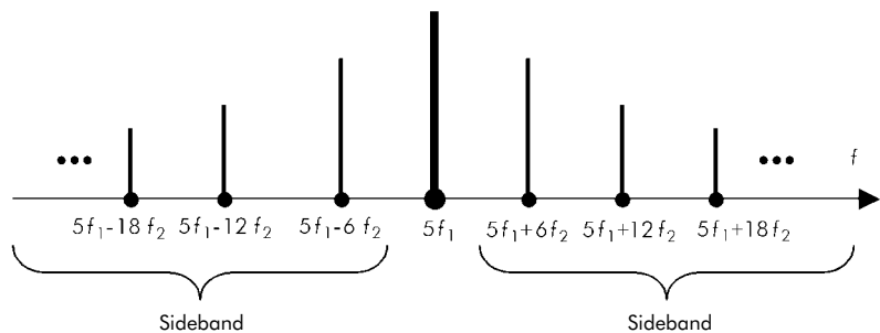
Figure 4 - Sidebands adjacent to the characteristic 5 th harmonic of a six-pulse converter P1 and P2
