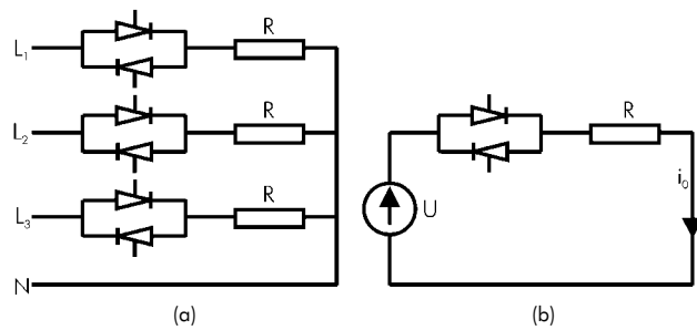
Figure 7 - Alternating current controller in a) a three-phase and b) a single-phase configuration
