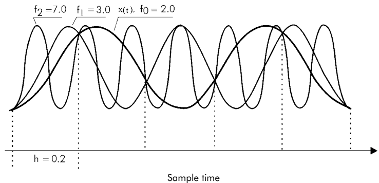
Figure A.2.2 - Analysis of ambiguity
