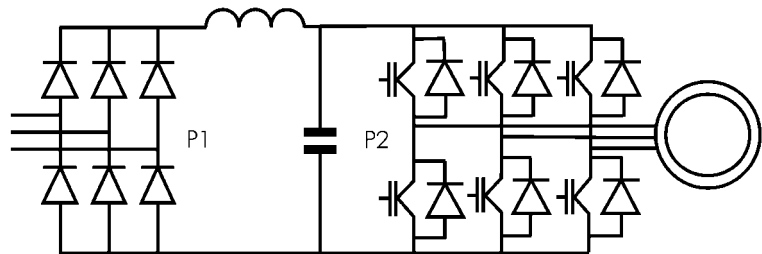
Figure 5 - Schematic diagram of a frequency converter with the voltage source dc-link
