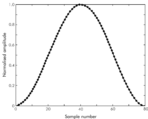
Figure A.1.6b - Hanning window
