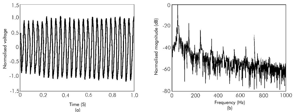
Figure 1 - Typical arc furnace voltage flicker measured at the supply transformer secondary a) fluctuation of voltage b) spectrum showing harmonics (spikes) and interharmonics [1]
