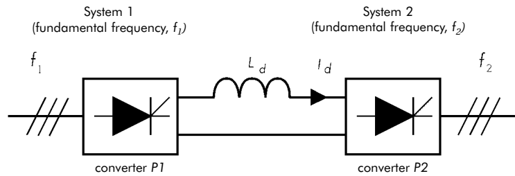
Figure 3 - Indirect frequency converter with a load commutated inverter
