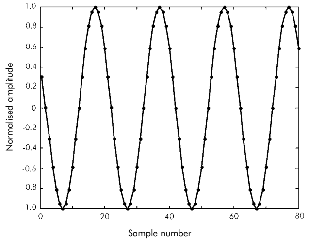
Figure A.1.4b - operation of the time window imposing y_i = w_i * x_i
